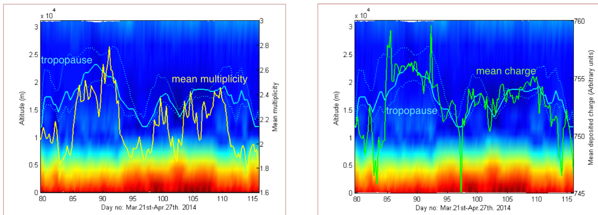
Figure 7. Time evolution of the tropopause altitude (light blue line; left axis) and several physical variables, between Mar. 21st. and Apr. 27th., 2014. The background color represents the temperature of the atmosphere: dark red for highest temperatures and dark blue for lowest temperatures. Left) Mean multiplicity (yellow line) evolution. Right) Mean charge (green line) evolution.
