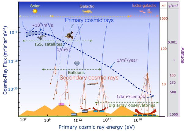
Figure 1. Energy spectrum (dark blue dashed line; left scale) of primary cosmic rays together with their corresponding estimated sources and the main detection techniques at different altitudes (right scale)
